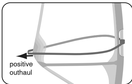
Fig. 5: Positive outhaul
